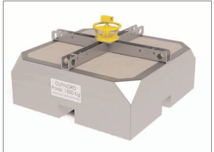
Concrete ballast with metal structure
